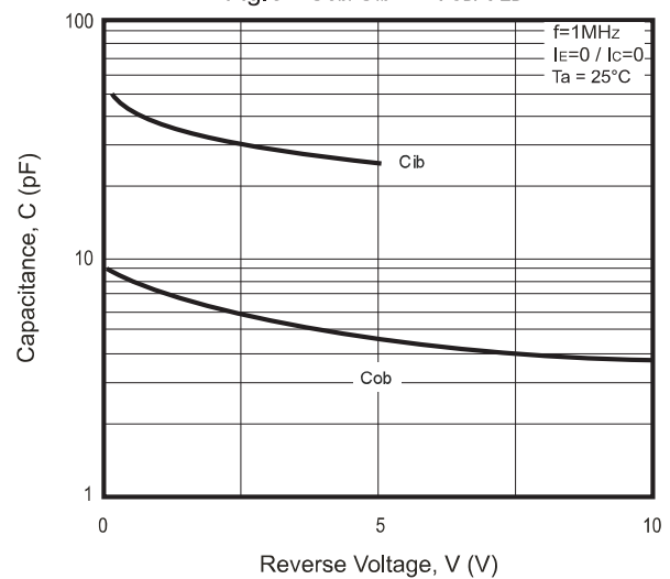
Fig.6 - C_{ob}/C_{ib} - V_{CB}/V_{EB}
