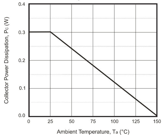
Fig.8 - P_C - T_a
